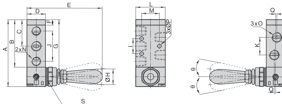
514.2000–514.2003 (5/3-Wege)
